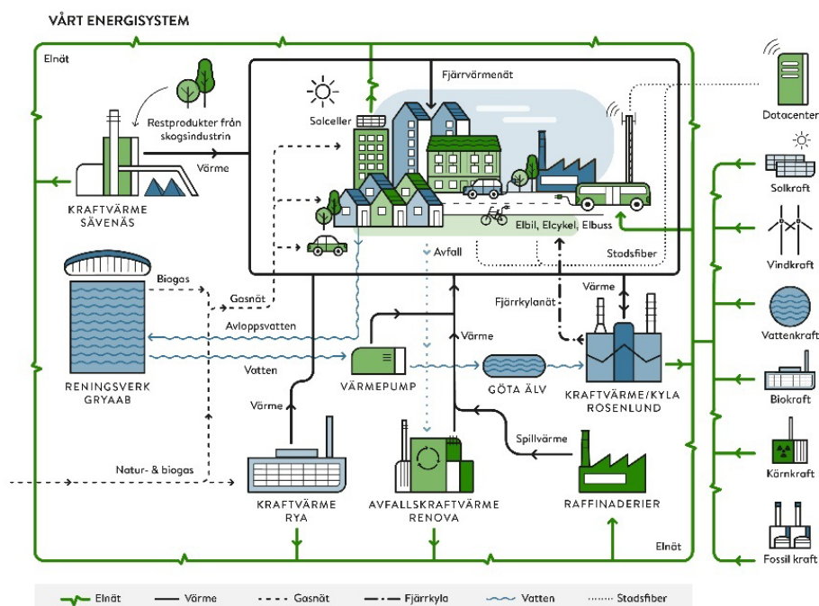
Figur 2. Energisystemet i Göteborg.
