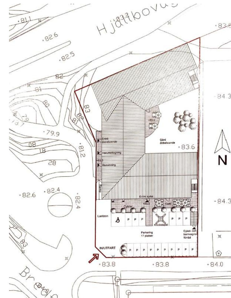
Situationsplan
