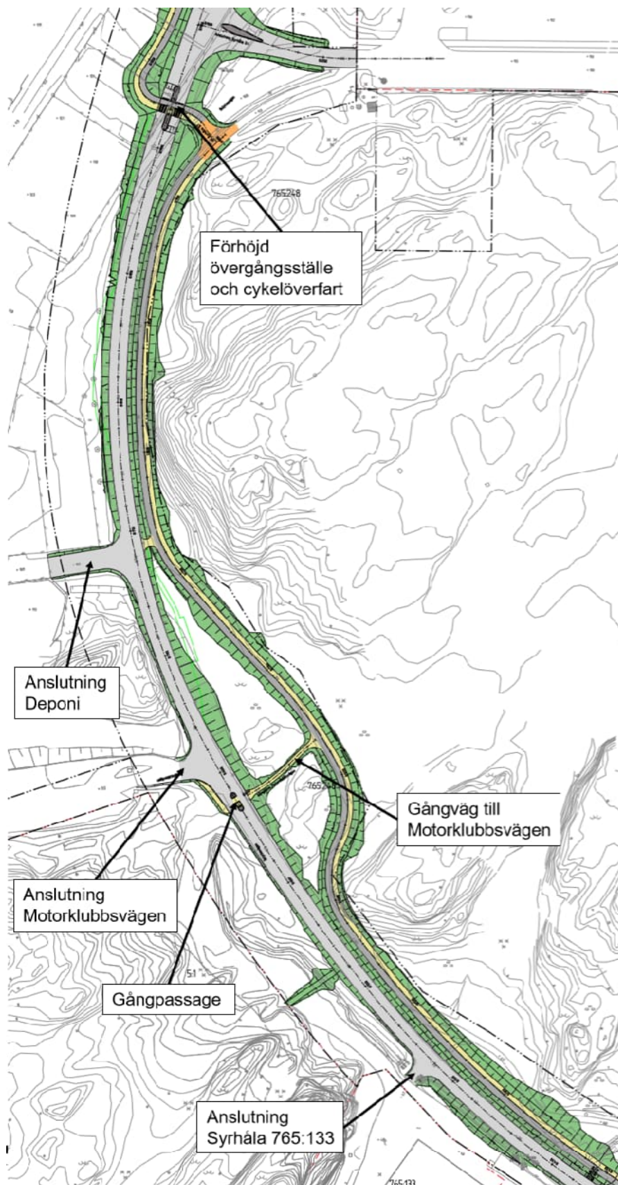
E.1:8 Planutformning 0/440-0/900.
