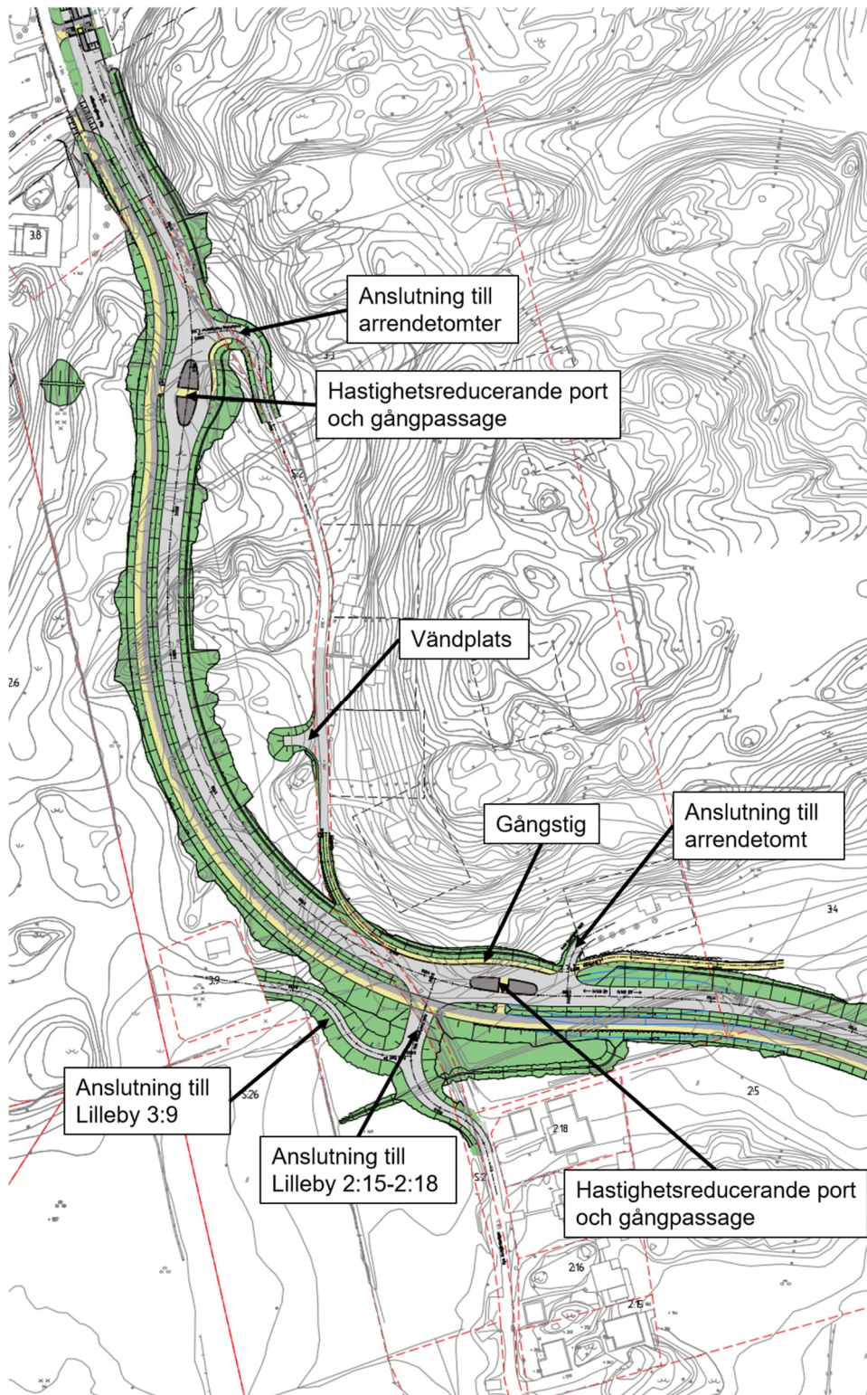
E.1:13 Planutformning 1/650-2/100.
