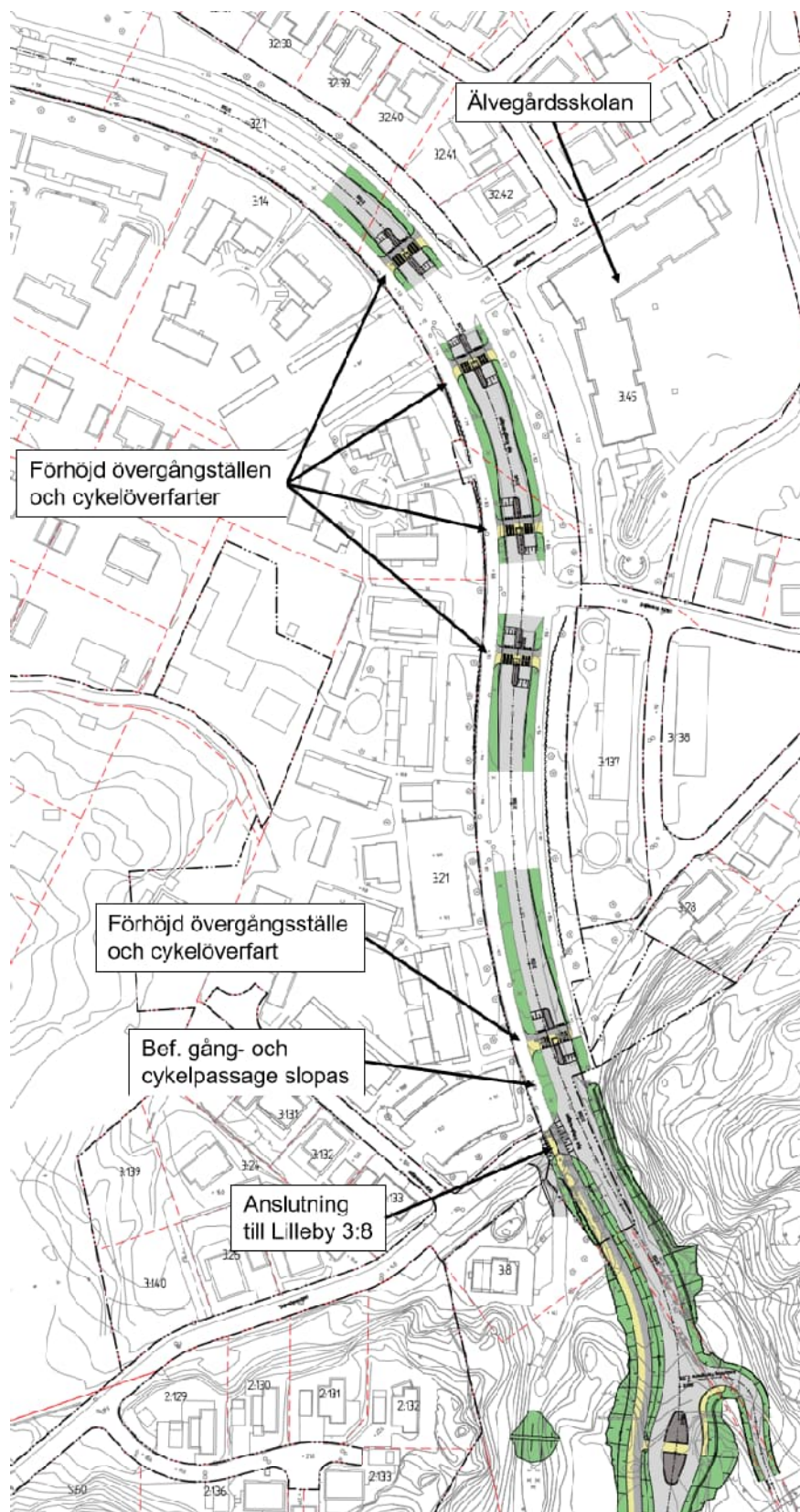
E.1:15 Planutformning 2/100-2/745.
